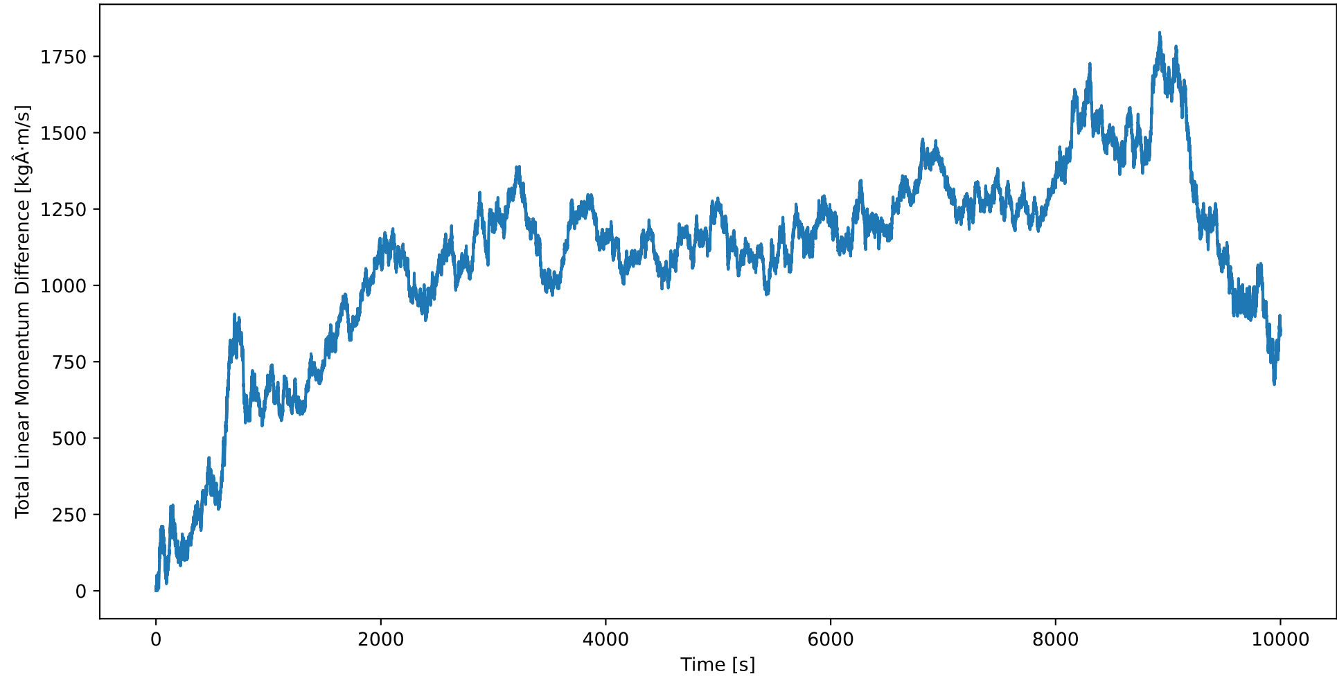
Total Linear Momentum Drift over time
